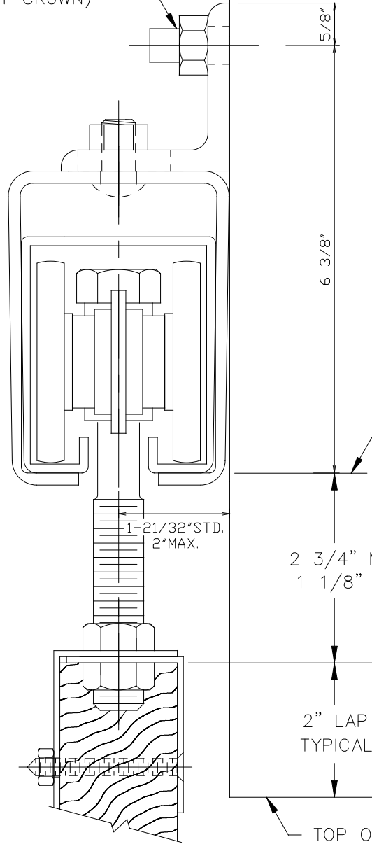
STANDARD HEAD SECTION USING SIDEWALL BRACKET
