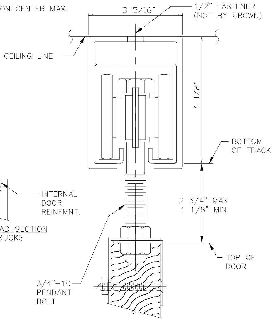
STANDARD HEAD SECTION USING OVERHEAD BRACKET
